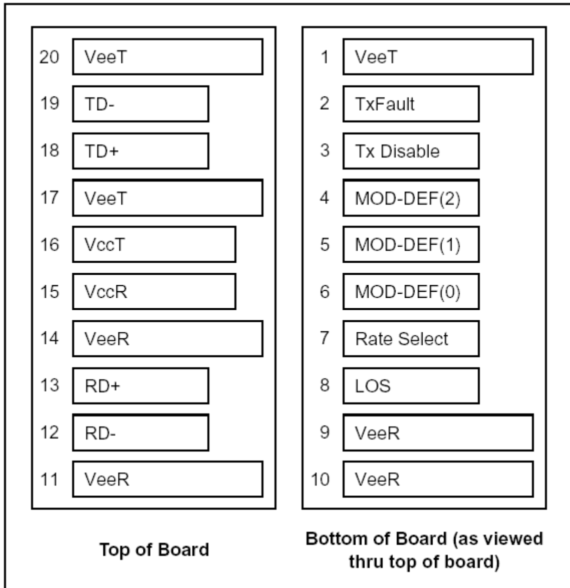
Figure 1. Pin Definitions
