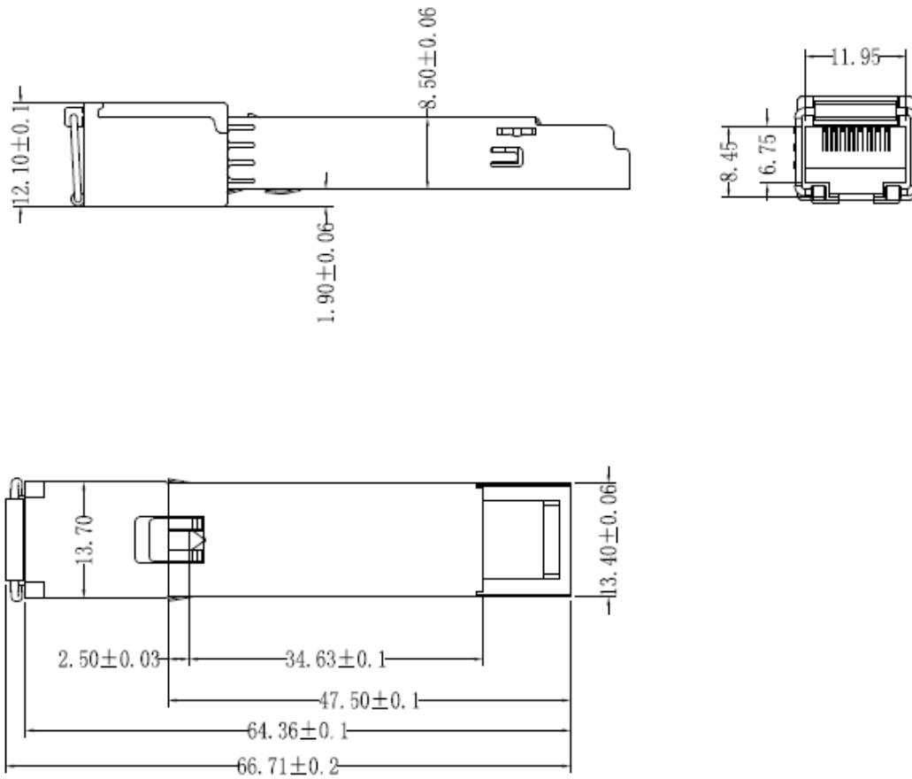
Figure 2. Mechanical dimensions
